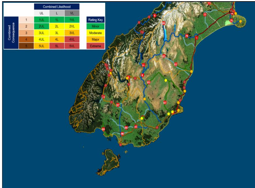
Figure 19: Map of Hazards with 2050 Risk Ratings
