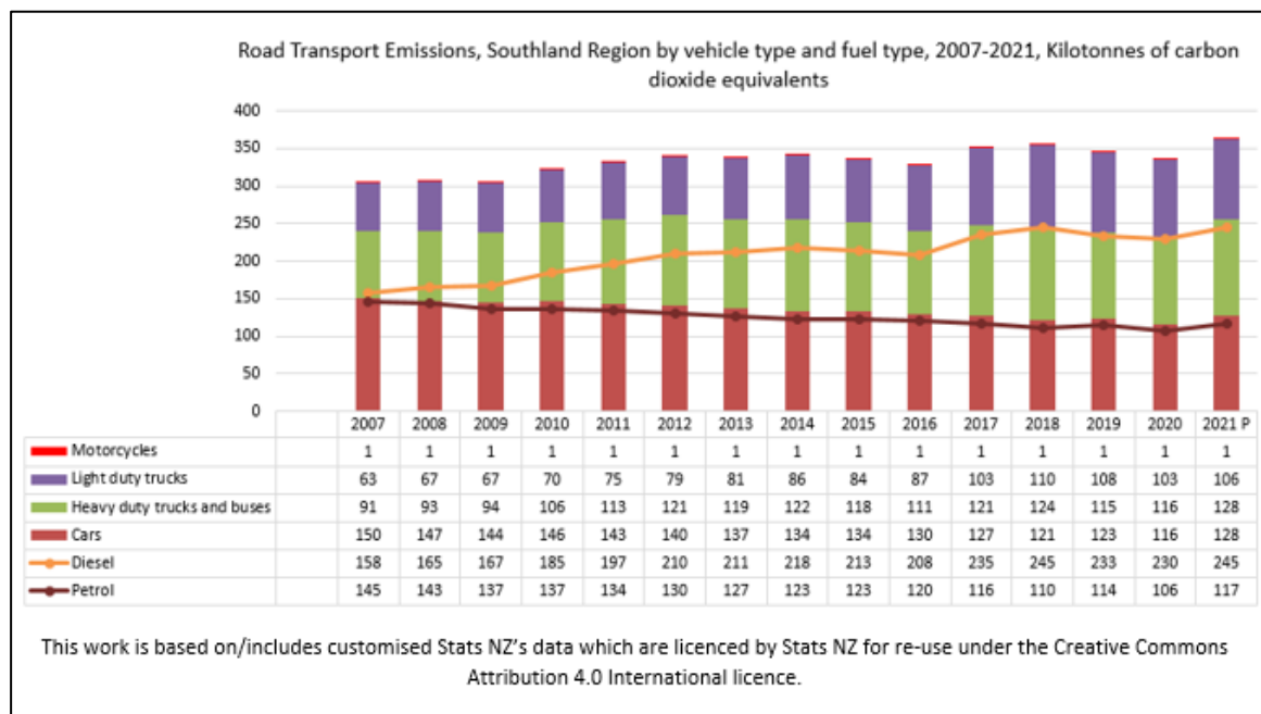
Figure 7: Transport Emissions for Southland
