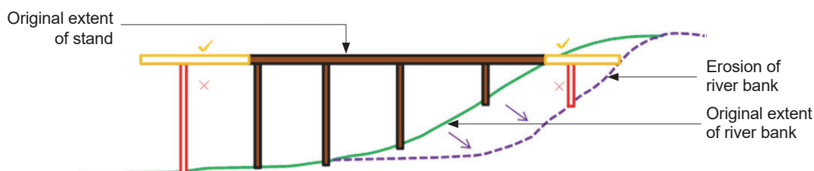
Figure 1: The gold sections show circumstances in which consent is not required to alter a whitebait stand. The red sections show circumstances in which consent is required to alter a whitebait stand.
