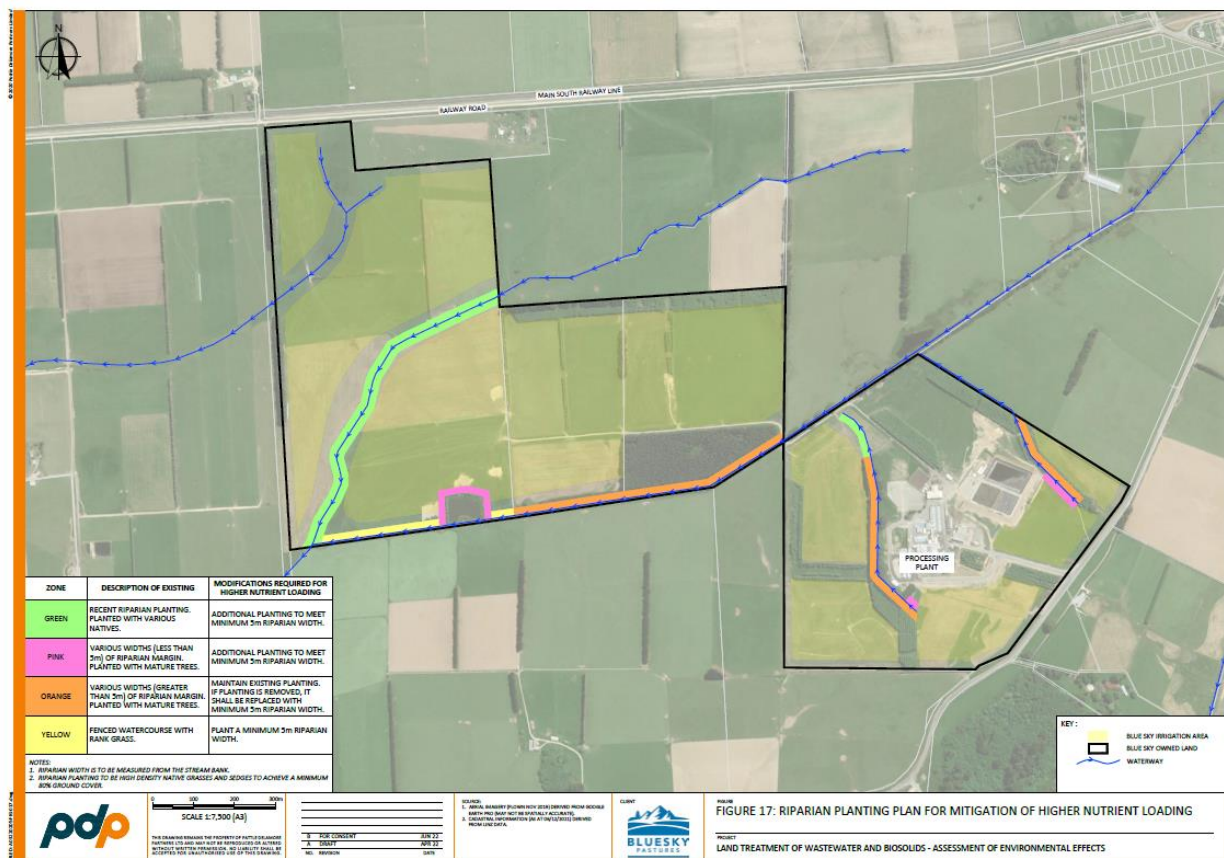
Figure 3-1: Existing and Proposed Planting Plan 4
