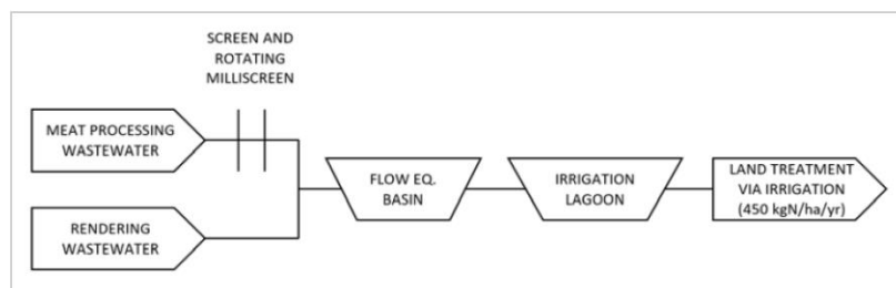
Figure 2-2: Process Diagram of Pre-2019 Wastewater System 1
