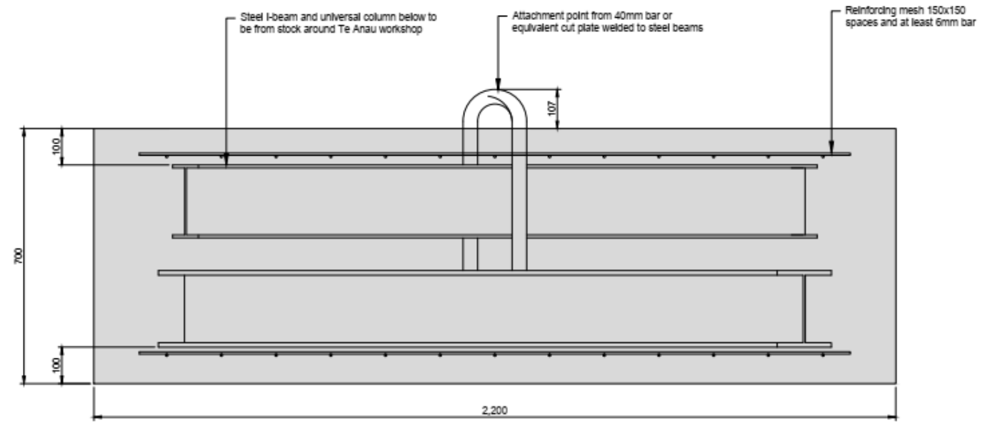
ANCHOR BLOCK ELEVATION
