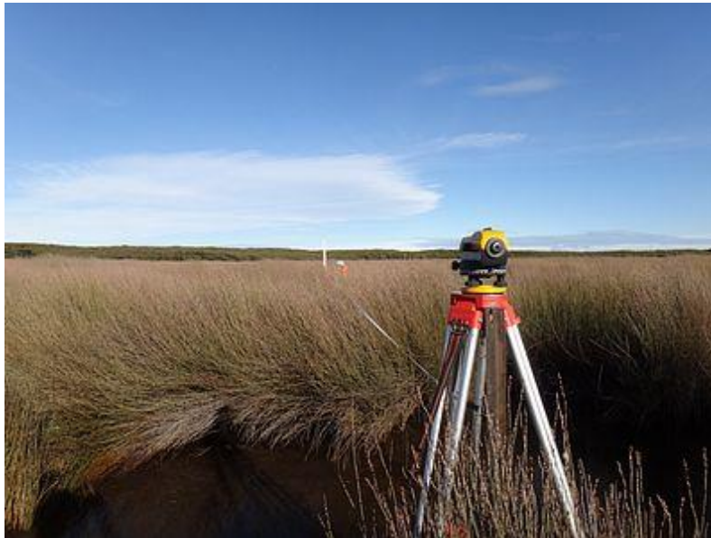
Photo 2: Using the builder's level to measure changes in elevation along T11_2012 (Bythell, 2012)
