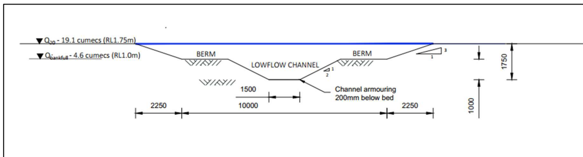
Figure 1 - Typical Shepherds Creek Diversion Profile
