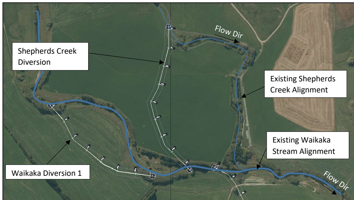
Figure 2 - Waikaka Stream and Shepherds Creek - Updated Diversion Locations
