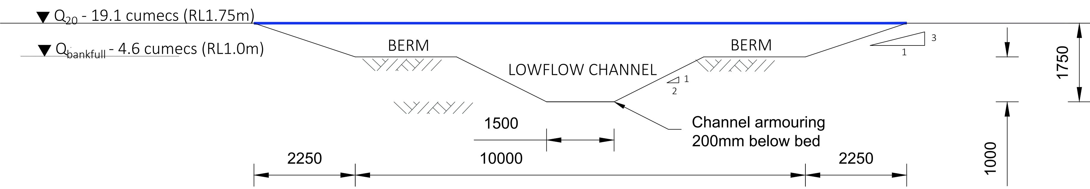
Typical Proposed Cross Section Shepherds Creek (Scale 1:100)
