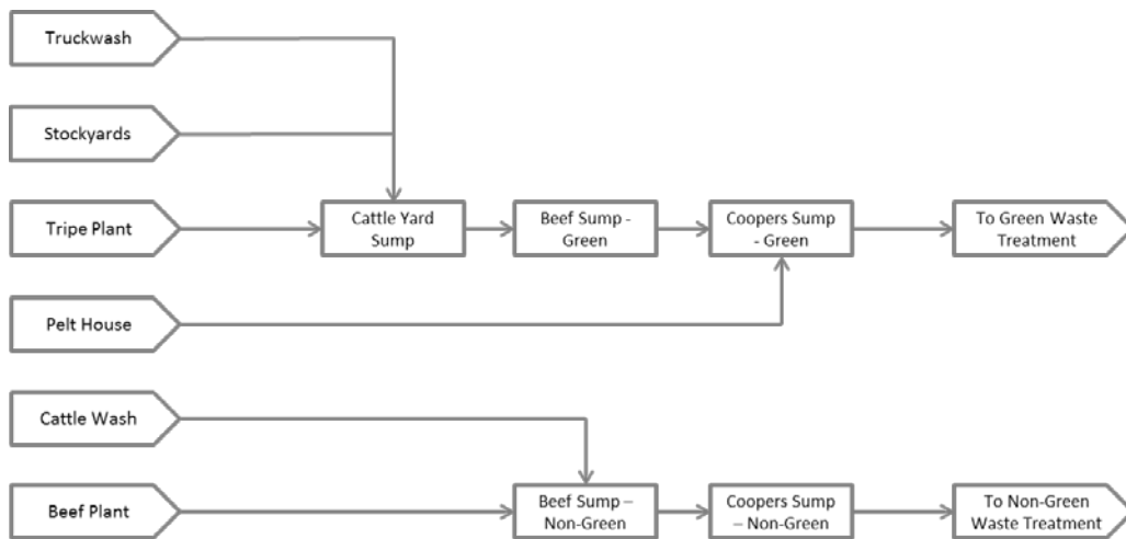
Figure 1: Main Plant Process Flow Diagram
