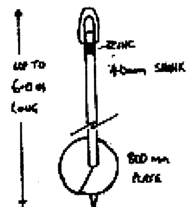
SCREW ANCHOR
