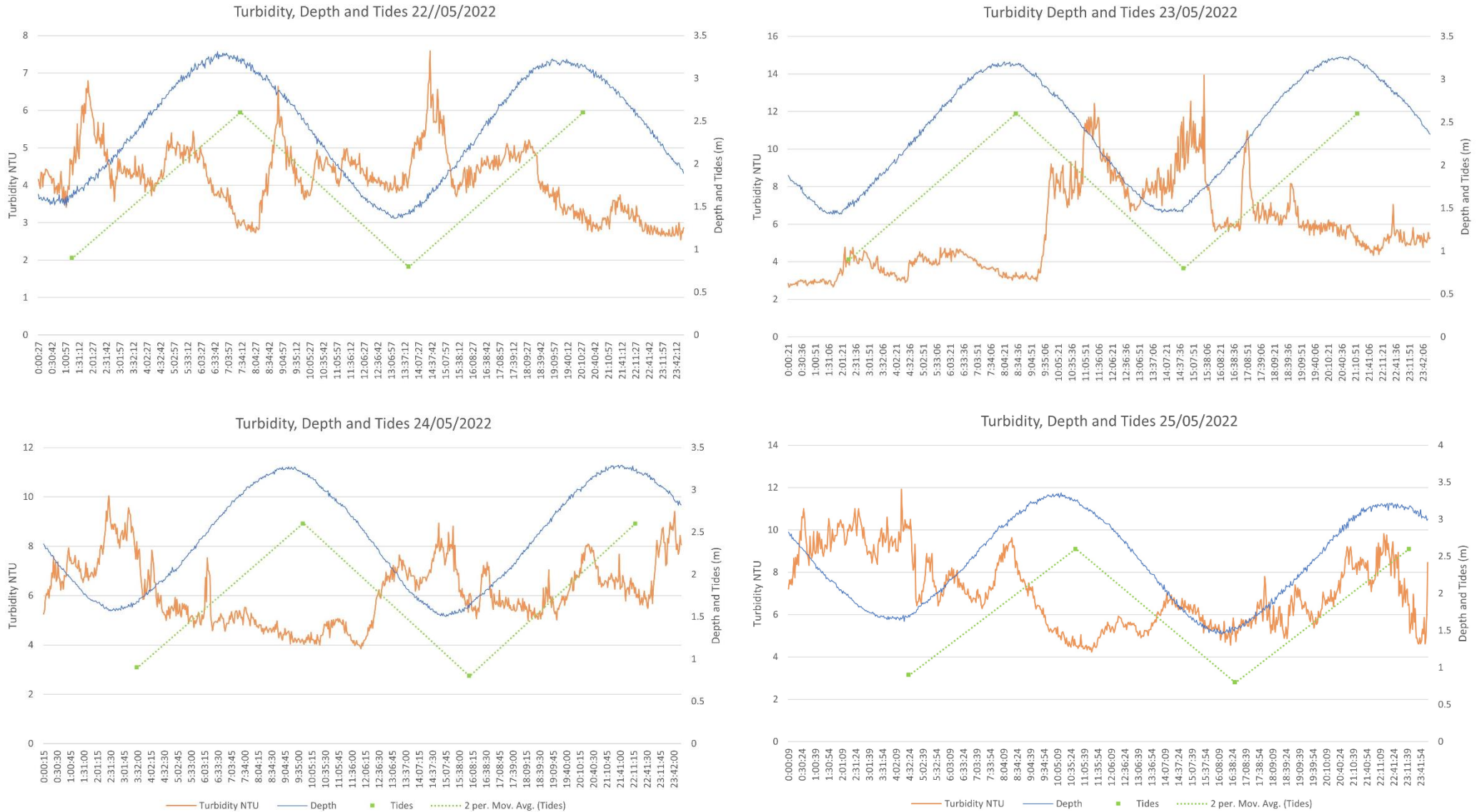
Figure 3: Tiwai Wharf seagrass site turbidity (NTU), tidal range/depth (m) and tidal cycle 22-25 May 2022.
