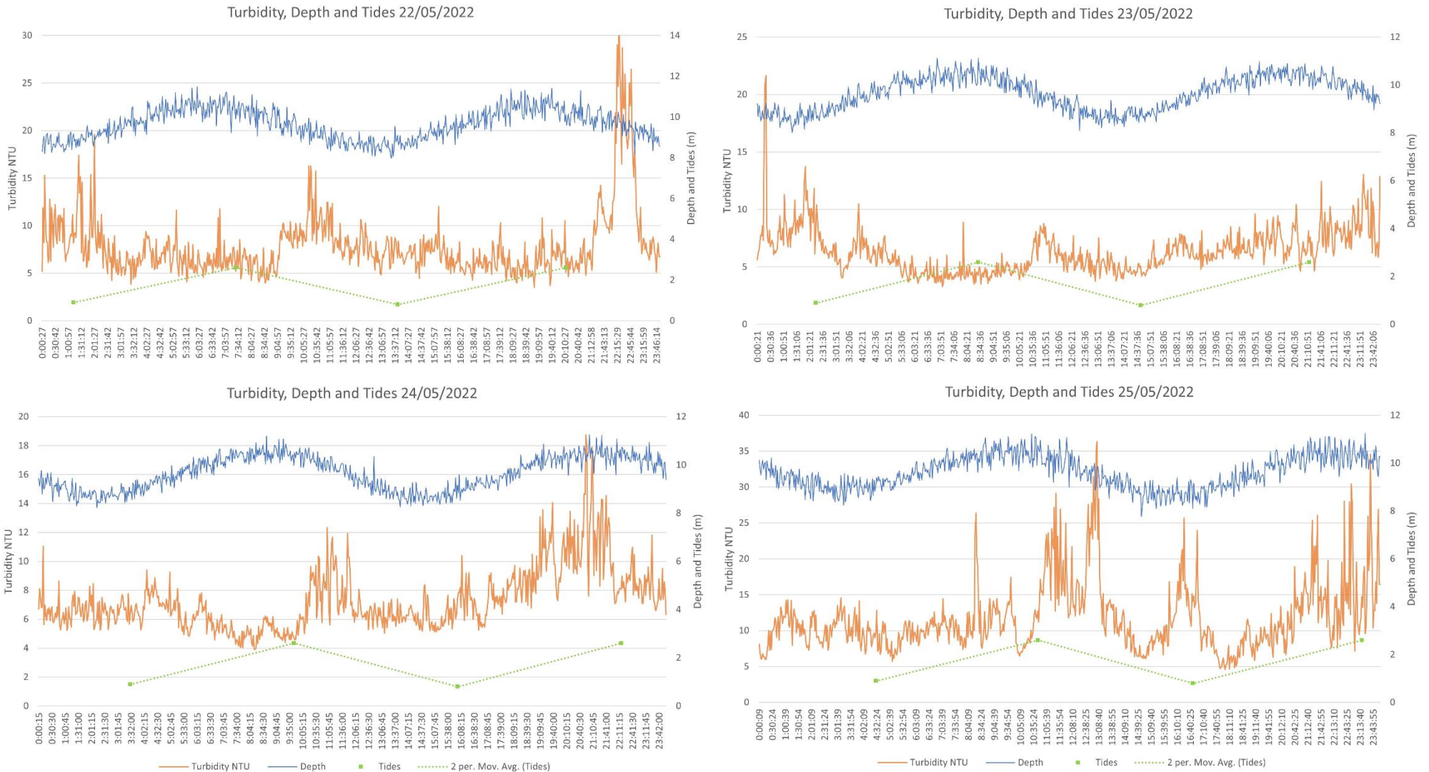
Figure 5: Disposal site turbidity (NTU), tidal range/depth (m) and tidal cycle 22-25 May 2022.
