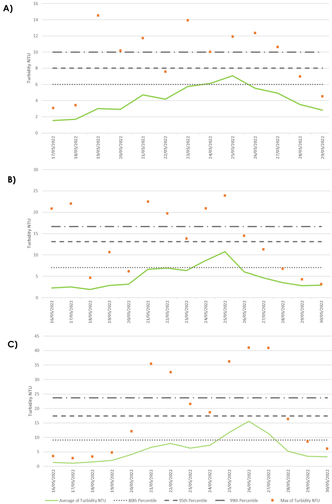
Figure 8: A) Tiwai wharf seagrass site; B) Rabbit Island seagrass site; and Disposal site daily turbidity (NTU) average and maximum with 80 th , 95 th and 99 th percentile daily average levels.
