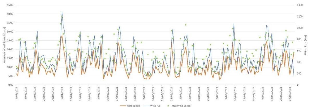
Figure 7: Daily averaged wind speed (knts), wind run (km) and maximum wind speed (knts) in Bluff Harbour between March and September 2021. (data from Tiwai Station, NIWA).
